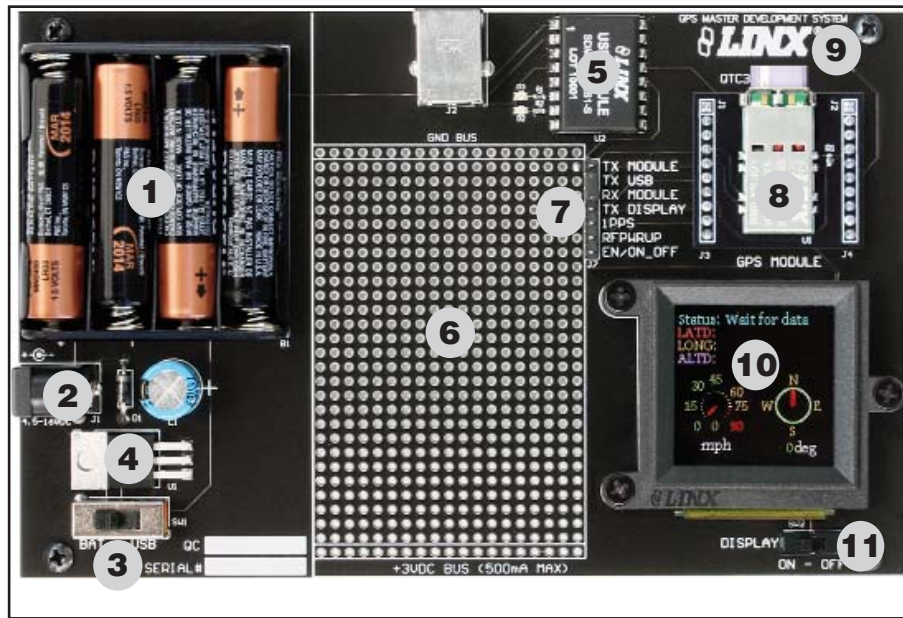
Figure 1: SR Series Receiver Development Board
