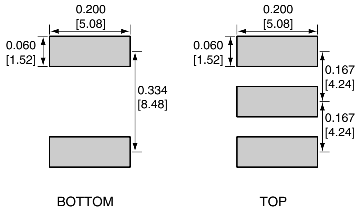
RECOMMENDED FOOTPRINT
