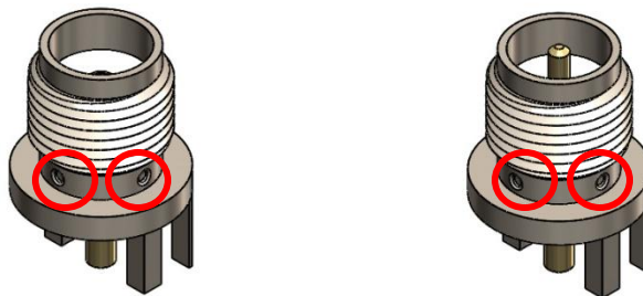
Figure 2: CONSMA003.062 and CONREVSMA003.062 with insulation retention dimples
